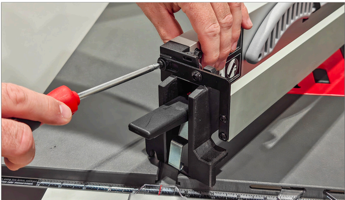
Step 1C. Remove Phillips Head Screw holding the Stock Support Bar to the SawStop Fence Assembly . Repeat on the other side of the fence.
