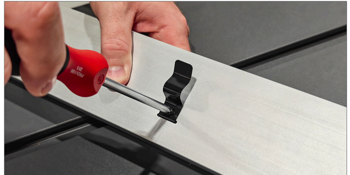
Step 1G. Remove Phillips Head Screw attaching the Push Stick Storage Tab on back of SawStop Fence Extrusion .
