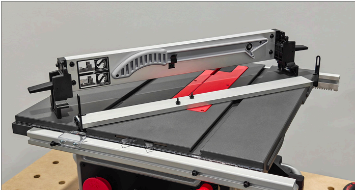
Step 1D. Remove the Stock Support Bar and set aside.
