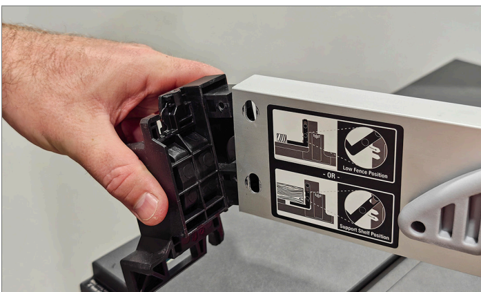
Step 1F. Remove the bracket from the SawStop Rip Fence extrusion by pulling it out. Repeat for the other bracket on the opposite side of the fence.
