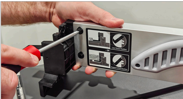
Step 1E. Remove two Phillips Head Screws from the back of the SawStop Rip Fence bracket. Repeat for the other bracket on the opposite side of the fence. Retain Screws for reassembly.
